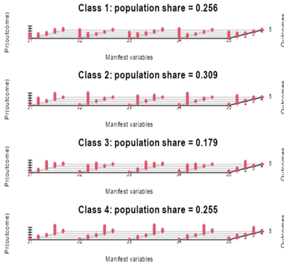
Figure 1. Item-Response Probabilities
